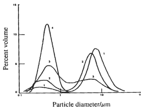
Figure 1: Variation in the size distribution of titanium dioxide dispersions with ionic strength at pH 8. (1) 10 -1 M, (2) 10 -2 M, (3) 10 -3 M, (4) 10 -4 M (Adapted from 7 ).
